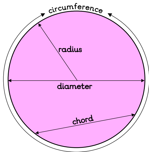
Parts of a circle
