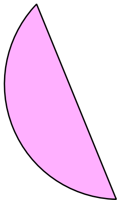
Segment of a circle
