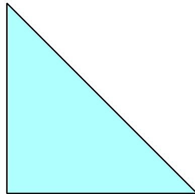
Right-angled isosceles triangle
